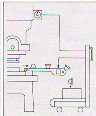
④カム入力・コンベア連動 Cam switch-belt conveyor interlocking operation.
